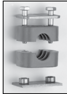
Fig. P1 – Weld Plate Assembly
