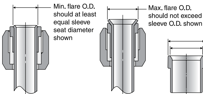
Fig. S29 — Comparing flare O.D. with sleeve seat and O.D.
