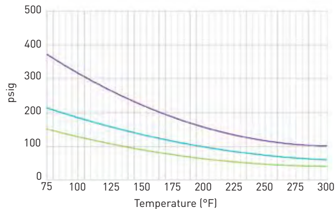
Retractable Coils PFA (Series 704) Maximum Working Pressure (psig)
